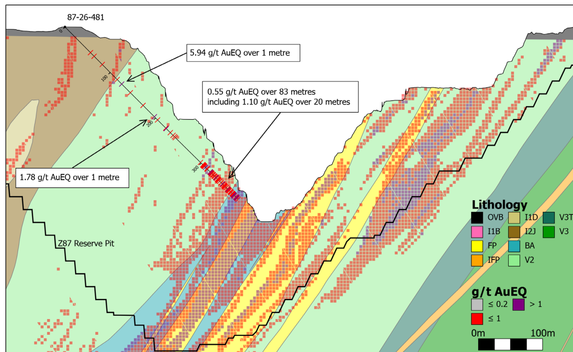
Figure 4. Cross section showing results for drillhole 87-26-481.
