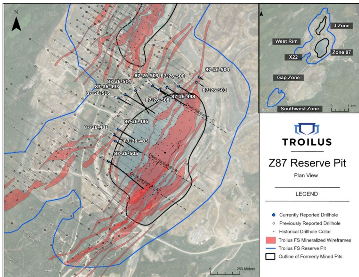
Figure 1. Plan Map with Reported Drill Hole and Cross Section Locations from Z87
