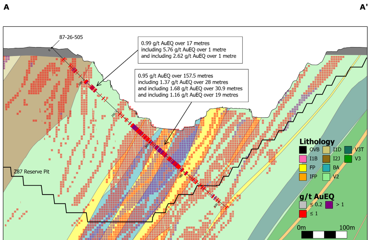
Figure 2. Cross section showing results for drillhole 87-26-505.
