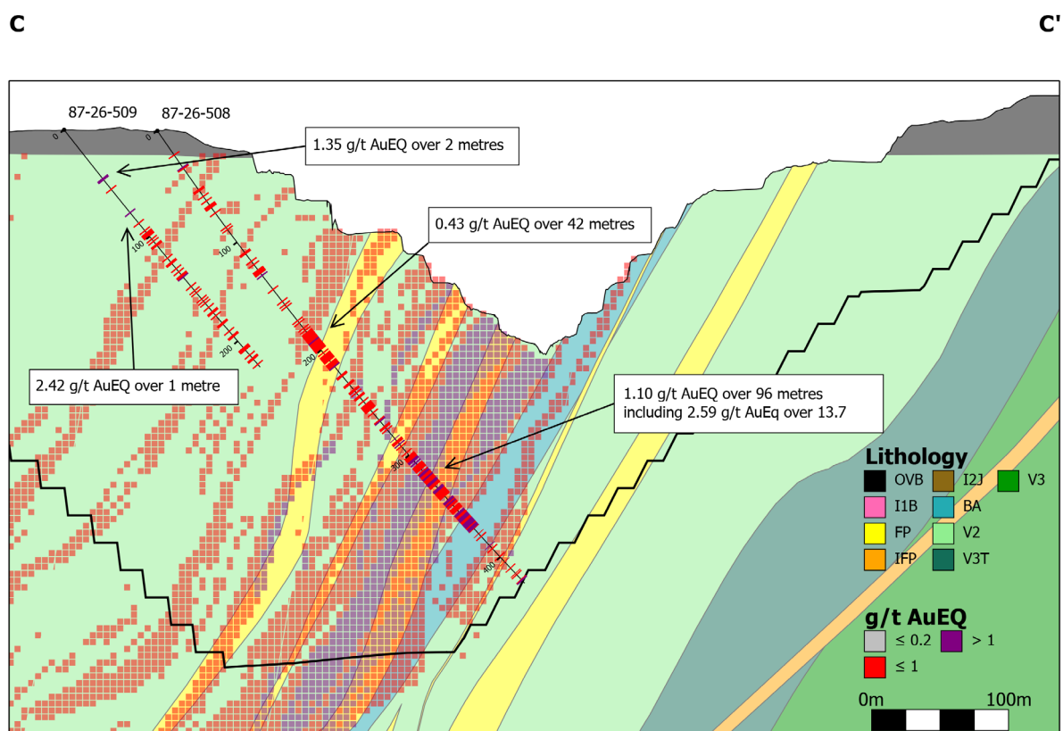
Figure 3. Cross section showing results for drillhole 87-26-508 and 87-26-509.
